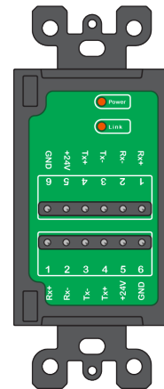
Terminated connector (back view)
