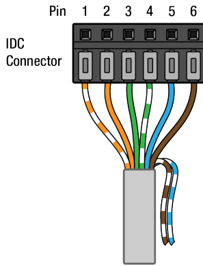
Cat 5
