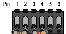
Terminated connector (back view)
